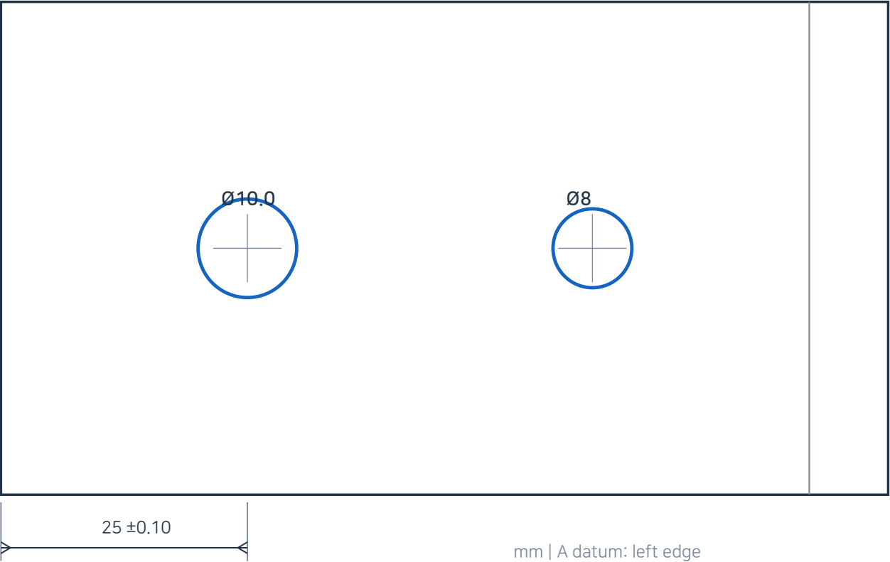
TOP VIEW — FOOTPRINT / HOLES
